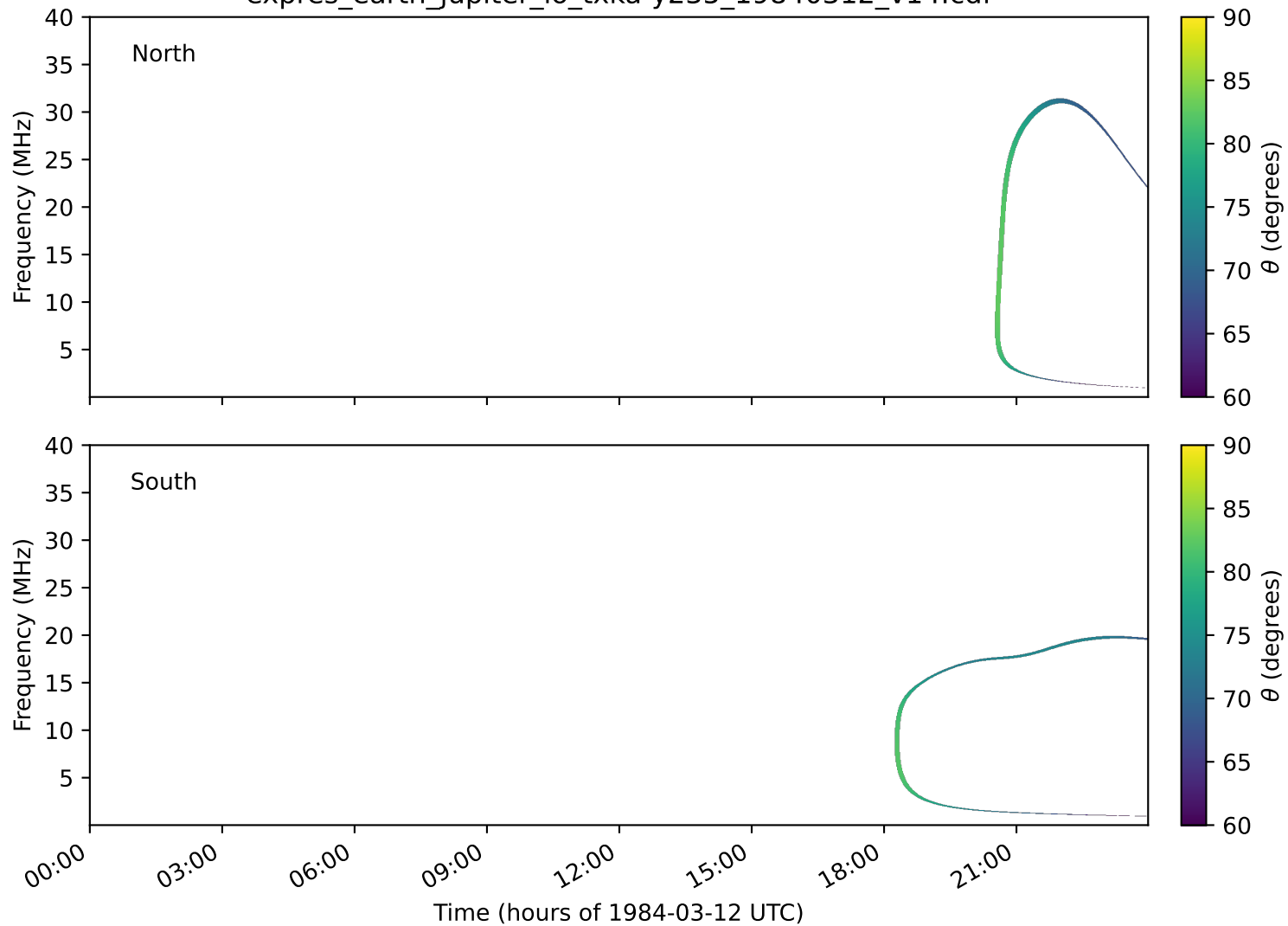
expres_earth_jupiter_io_txka-y235_19840312_v14.cdf
