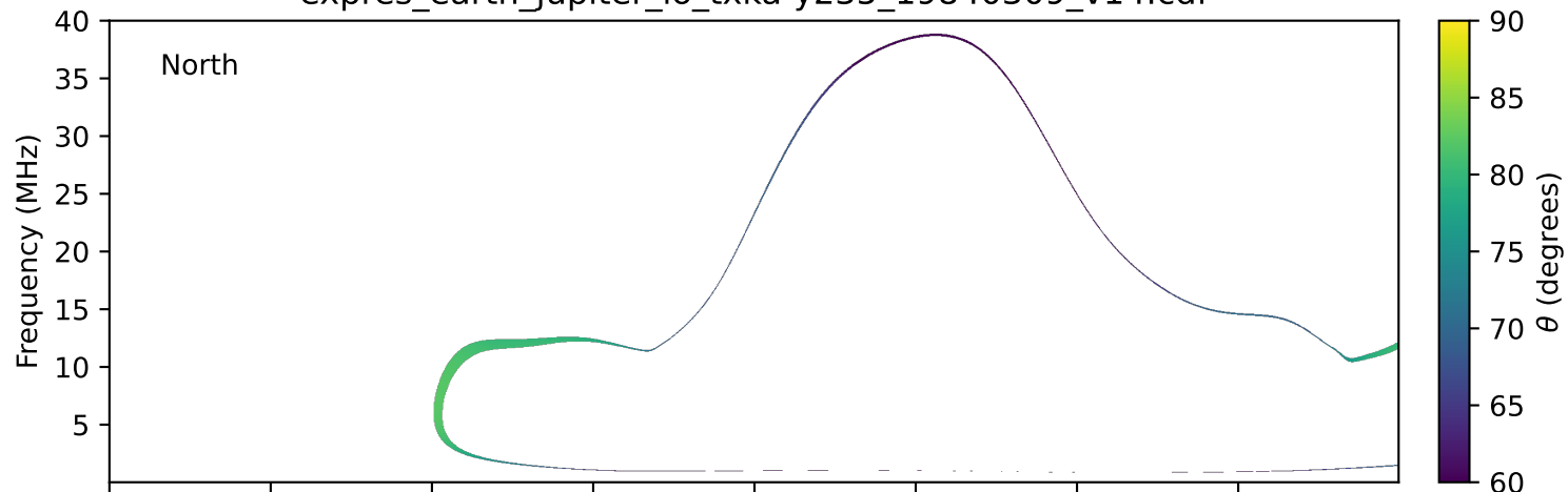
expres_earth_jupiter_io_txka-y235_19840309_v14.cdf
