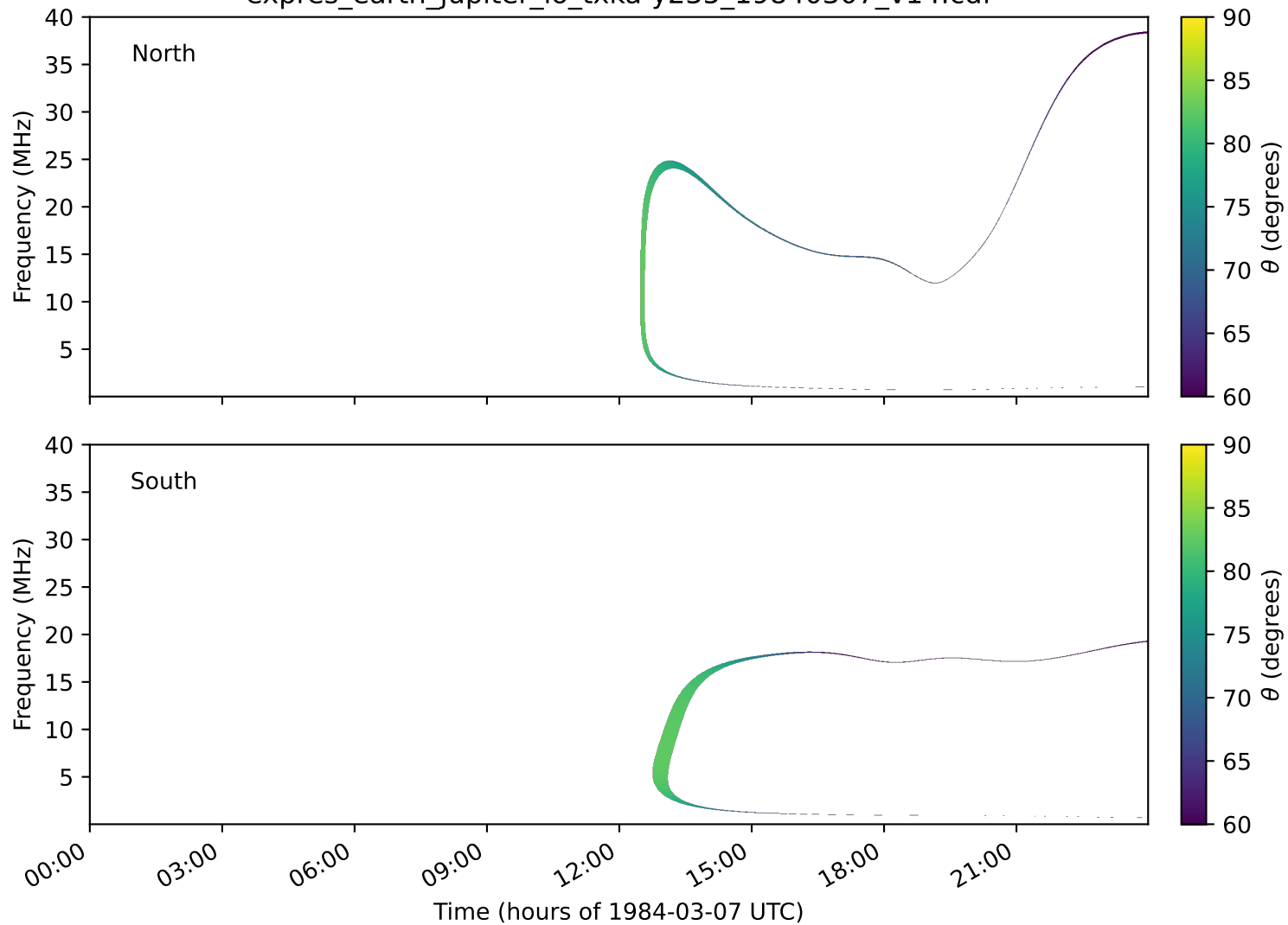
expres_earth_jupiter_io_txka-y235_19840307_v14.cdf
