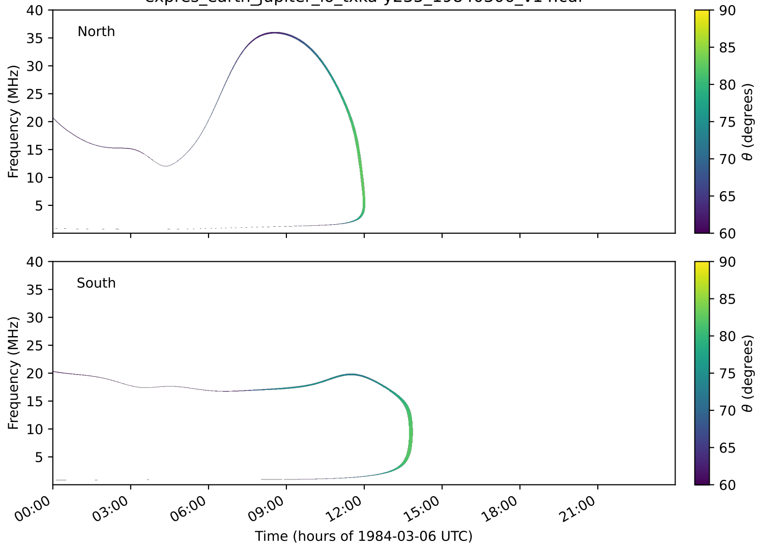
expres_earth_jupiter_io_txka-y235_19840306_v14.cdf
