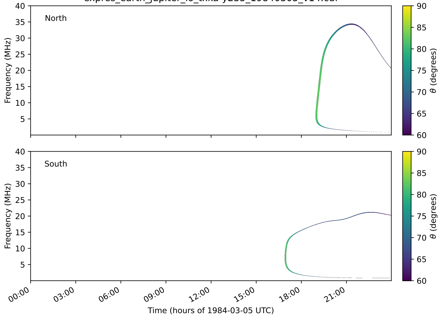
expres_earth_jupiter_io_txka-y235_19840305_v14.cdf
