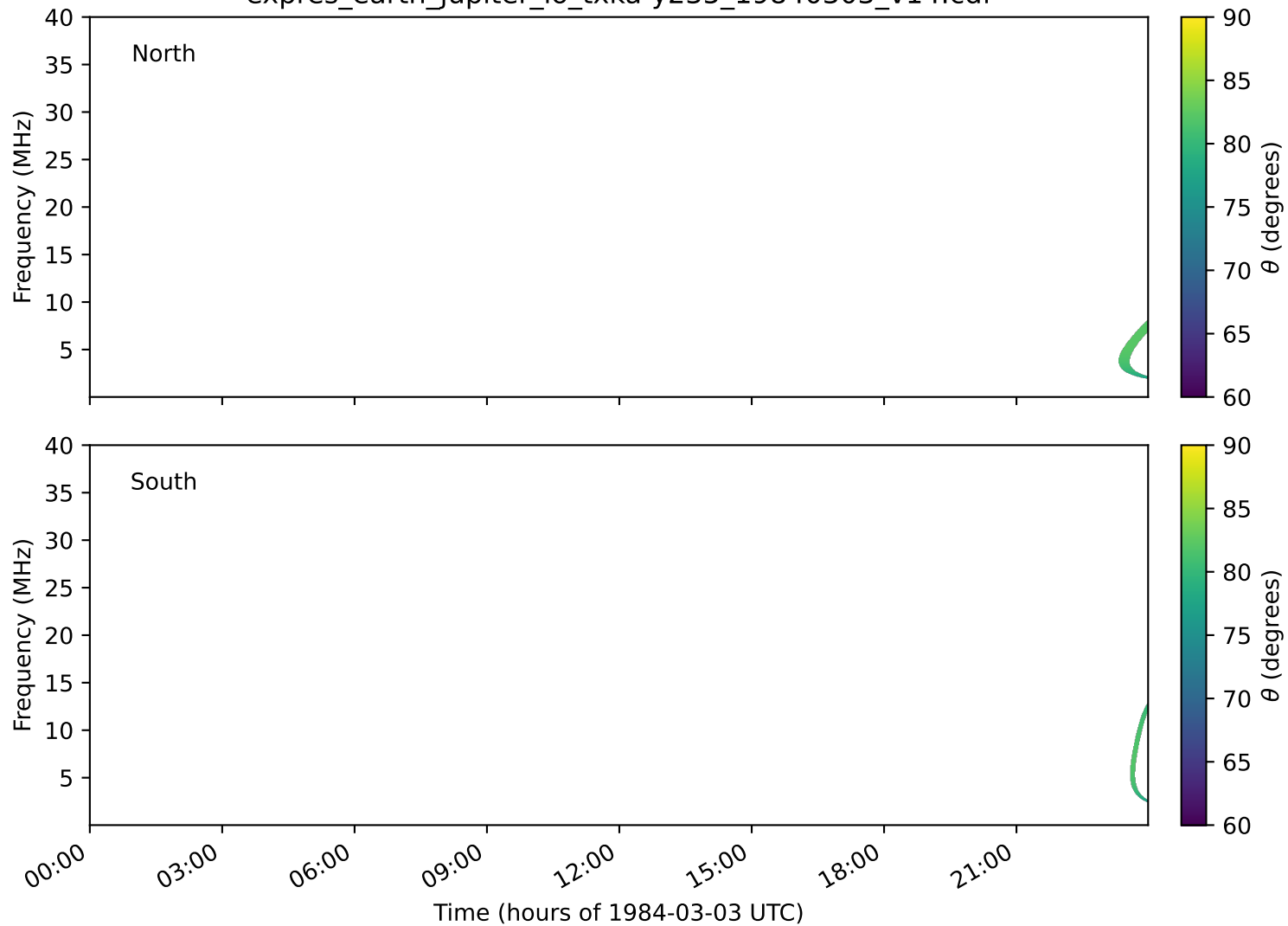
expres_earth_jupiter_io_txka-y235_19840303_v14.cdf
