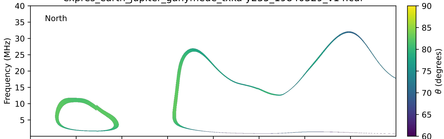
expres_earth_jupiter_ganymede_txka-y235_19840329_v14.cdf
