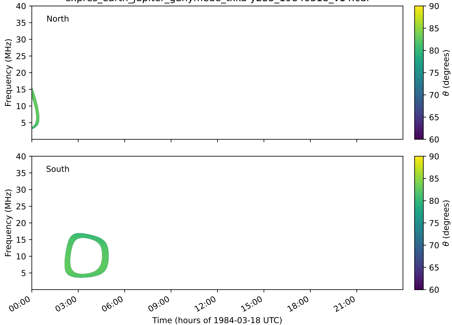
expres_earth_jupiter_ganymede_txka-y235_19840318_v14.cdf
