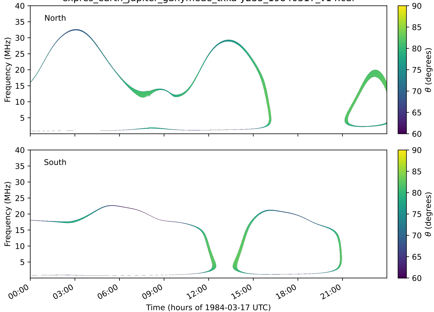
expres_earth_jupiter_ganymede_txka-y235_19840317_v14.cdf
