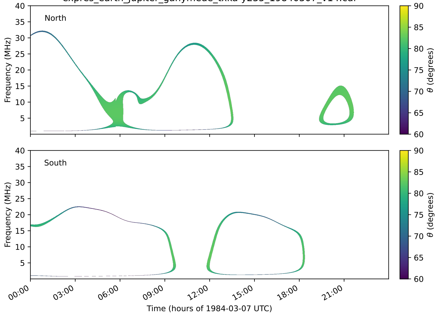
expres_earth_jupiter_ganymede_txka-y235_19840307_v14.cdf
