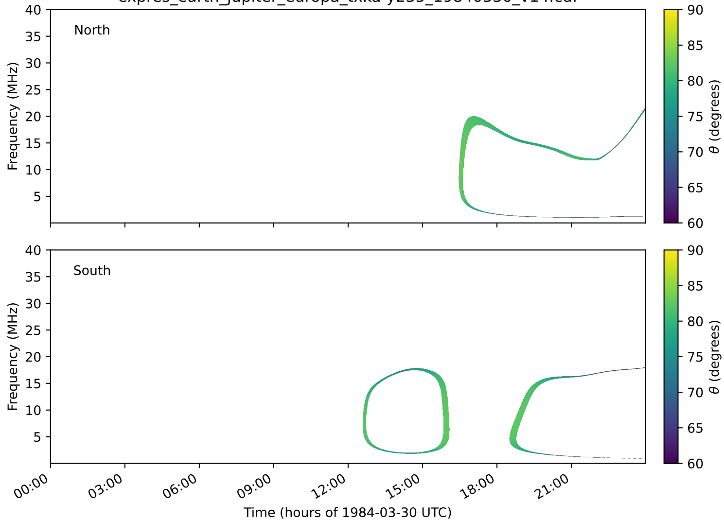
expres_earth_jupiter_europa_txka-y235_19840330_v14.cdf
