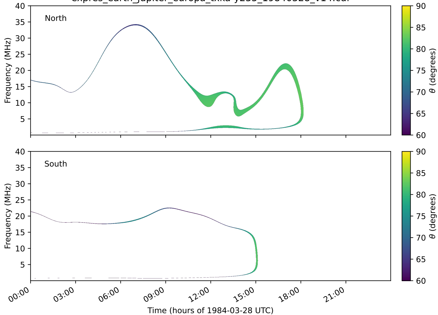
expres_earth_jupiter_europa_txka-y235_19840328_v14.cdf
