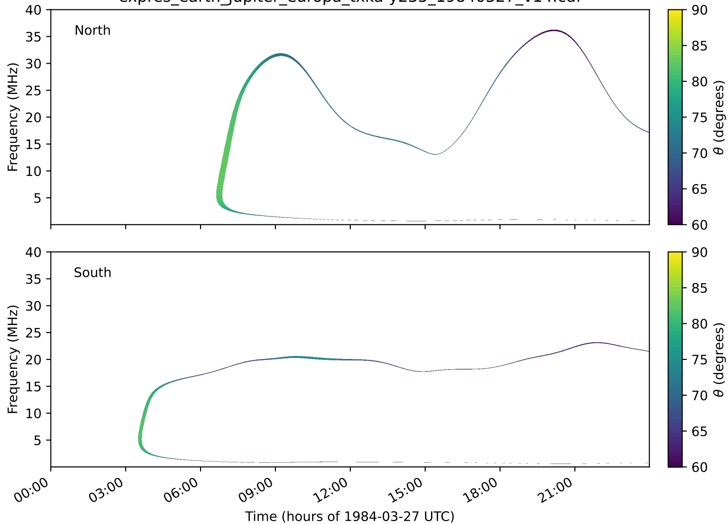
expres_earth_jupiter_europa_txka-y235_19840327_v14.cdf
