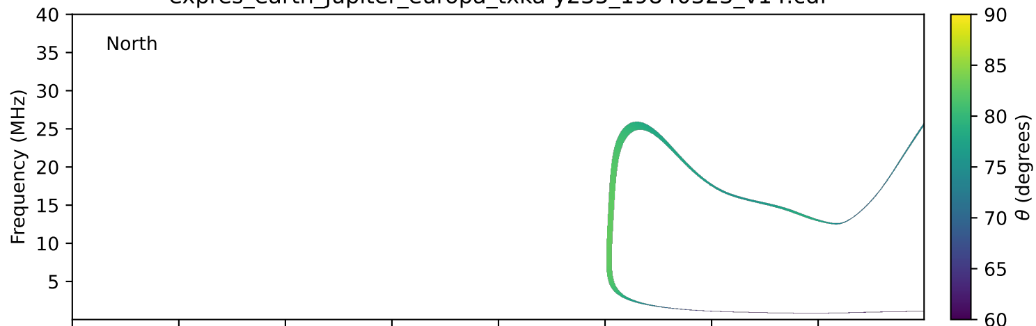
expres_earth_jupiter_europa_txka-y235_19840323_v14.cdf
