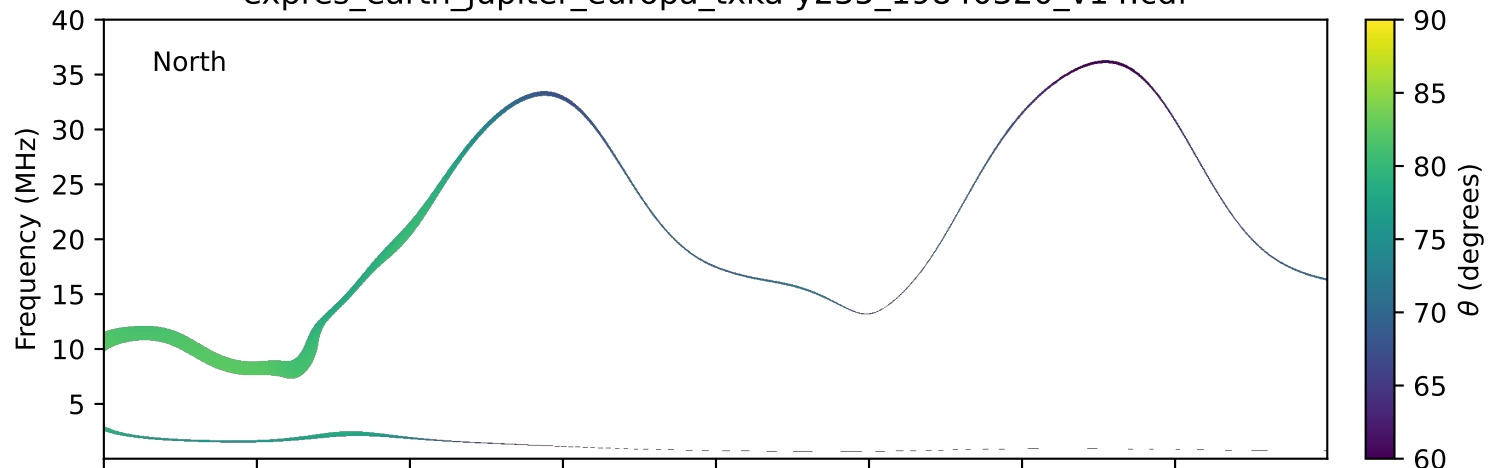
expres_earth_jupiter_europa_txka-y235_19840320_v14.cdf
