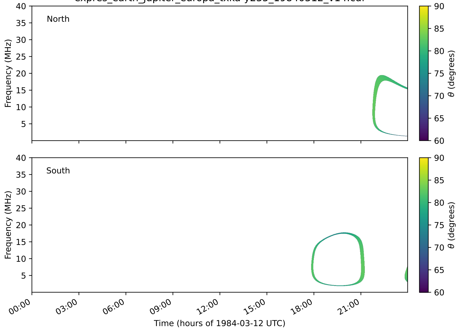
expres_earth_jupiter_europa_txka-y235_19840312_v14.cdf
