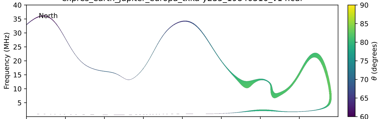
expres_earth_jupiter_europa_txka-y235_19840310_v14.cdf
