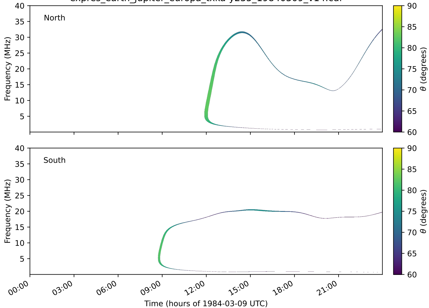
expres_earth_jupiter_europa_txka-y235_19840309_v14.cdf
