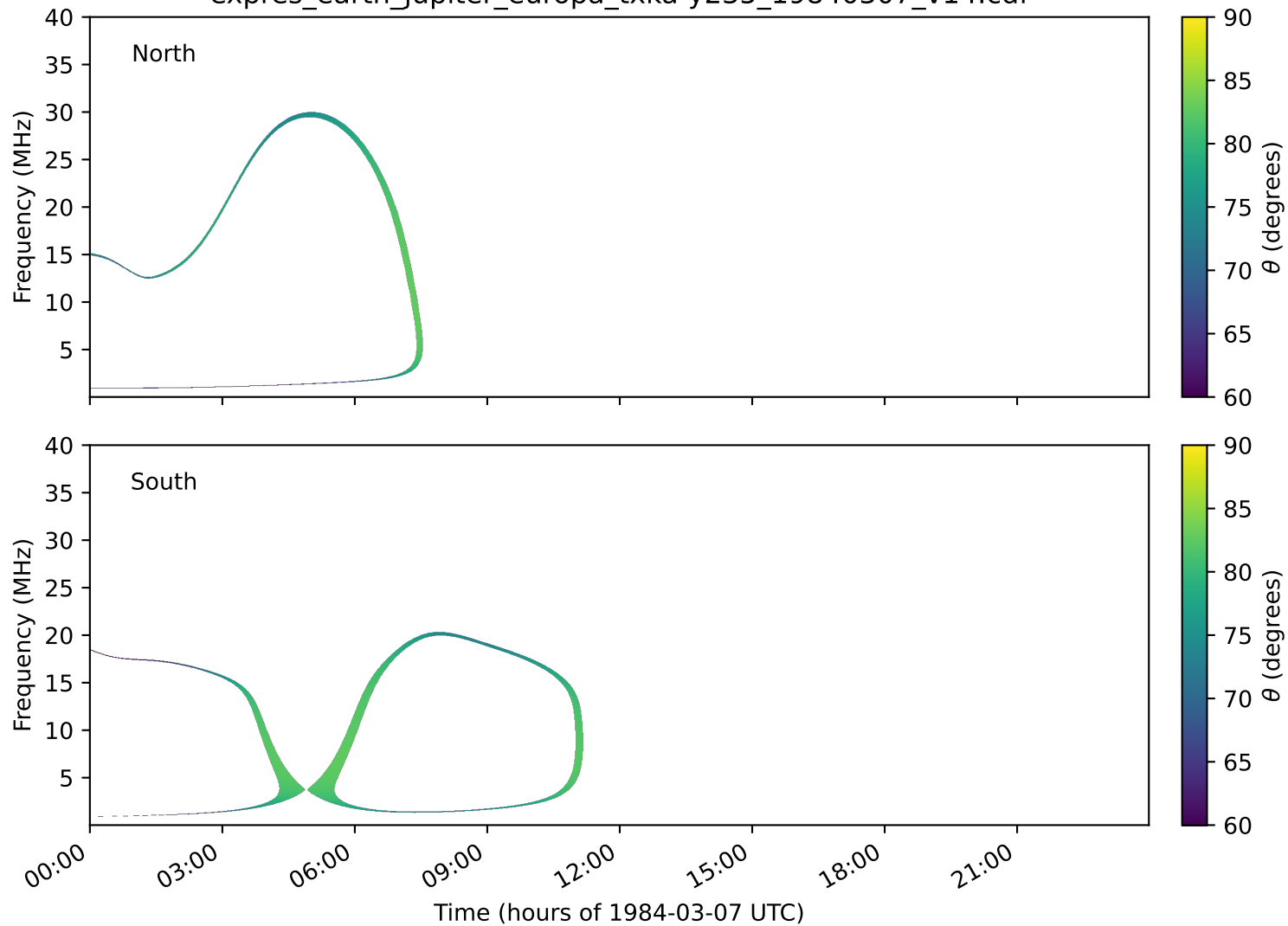
expres_earth_jupiter_europa_txka-y235_19840307_v14.cdf
