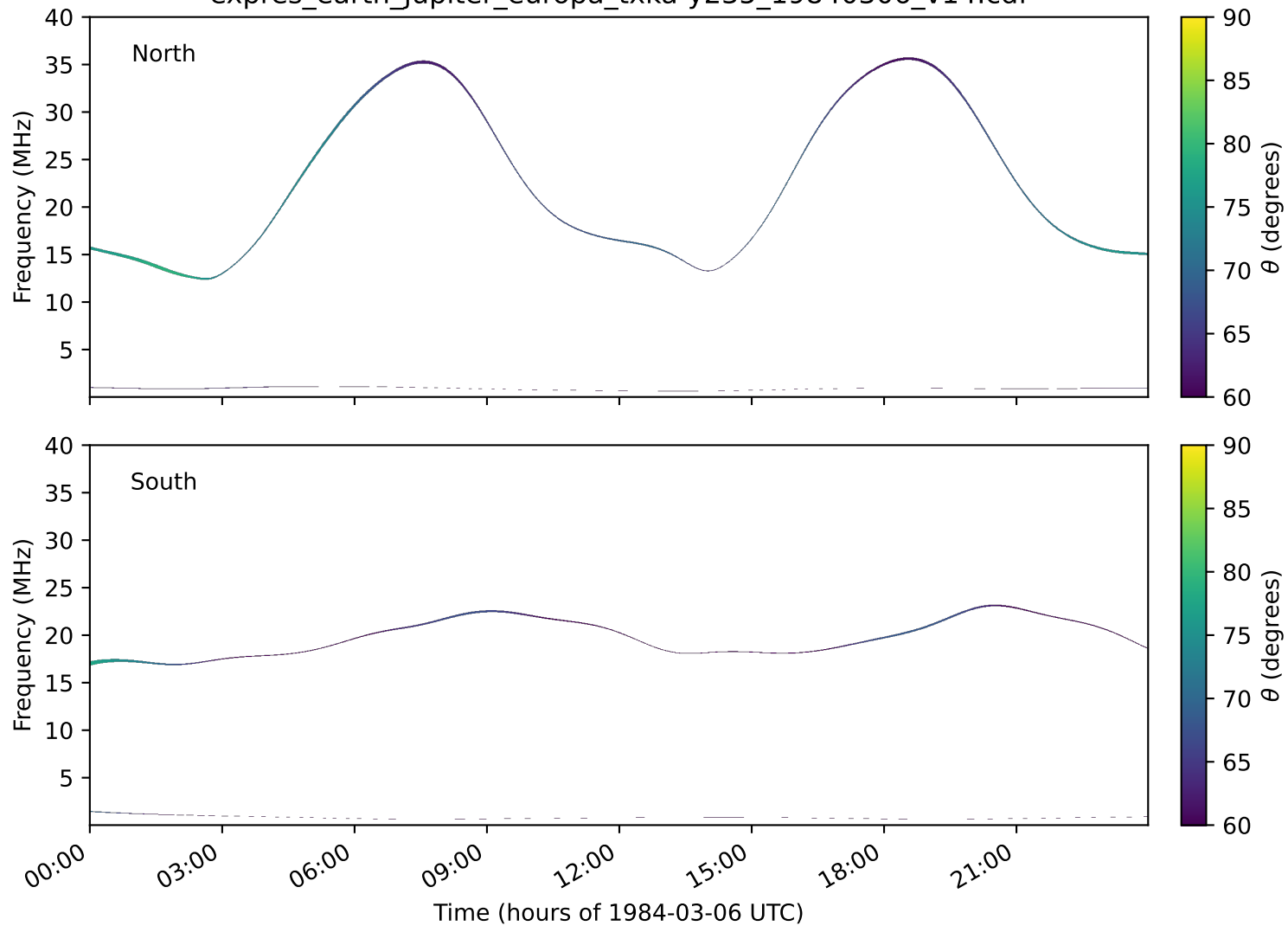
expres_earth_jupiter_europa_txka-y235_19840306_v14.cdf
