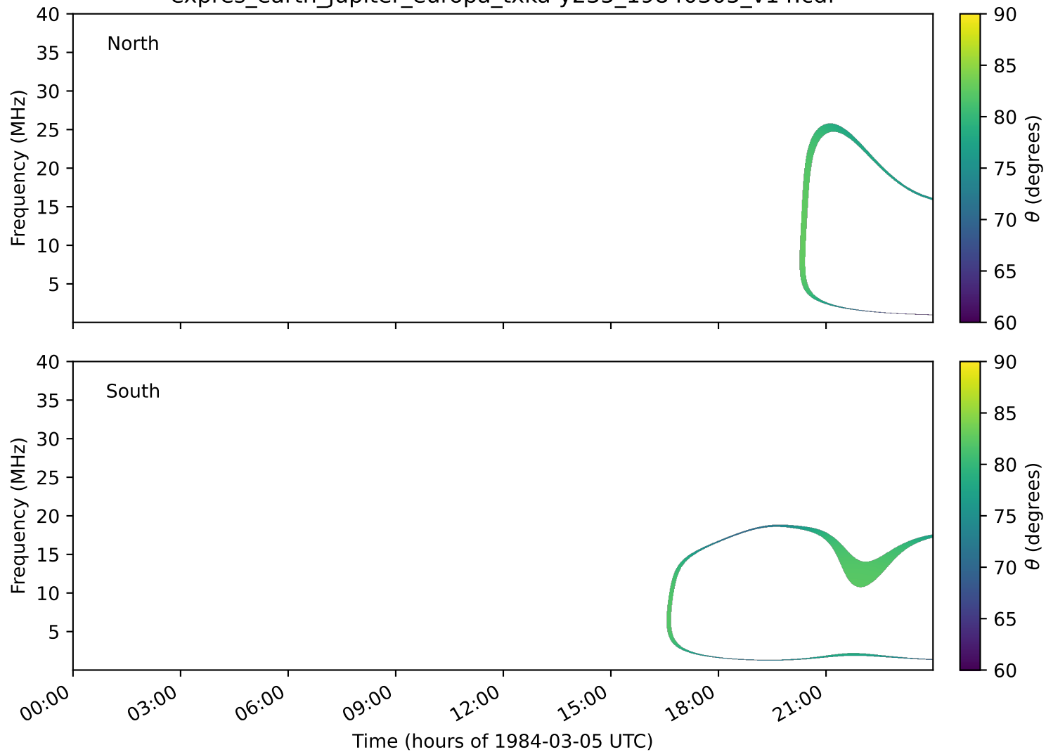
expres_earth_jupiter_europa_txka-y235_19840305_v14.cdf
