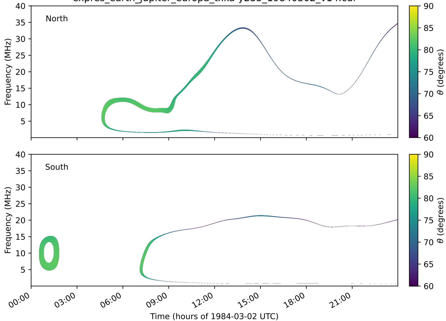
expres_earth_jupiter_europa_txka-y235_19840302_v14.cdf
