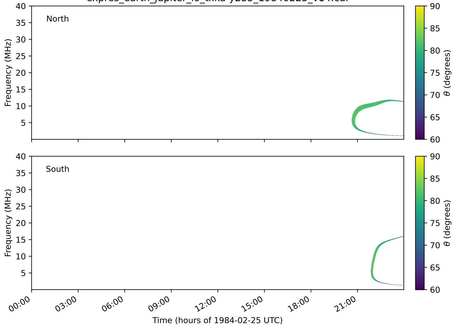
expres_earth_jupiter_io_txka-y235_19840225_v14.cdf
