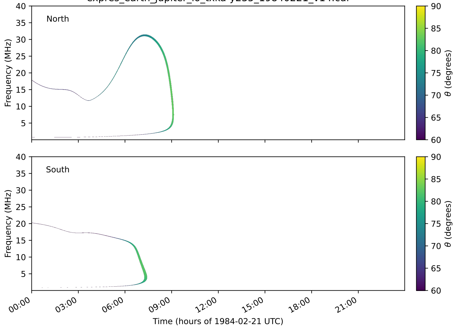
expres_earth_jupiter_io_txka-y235_19840221_v14.cdf
