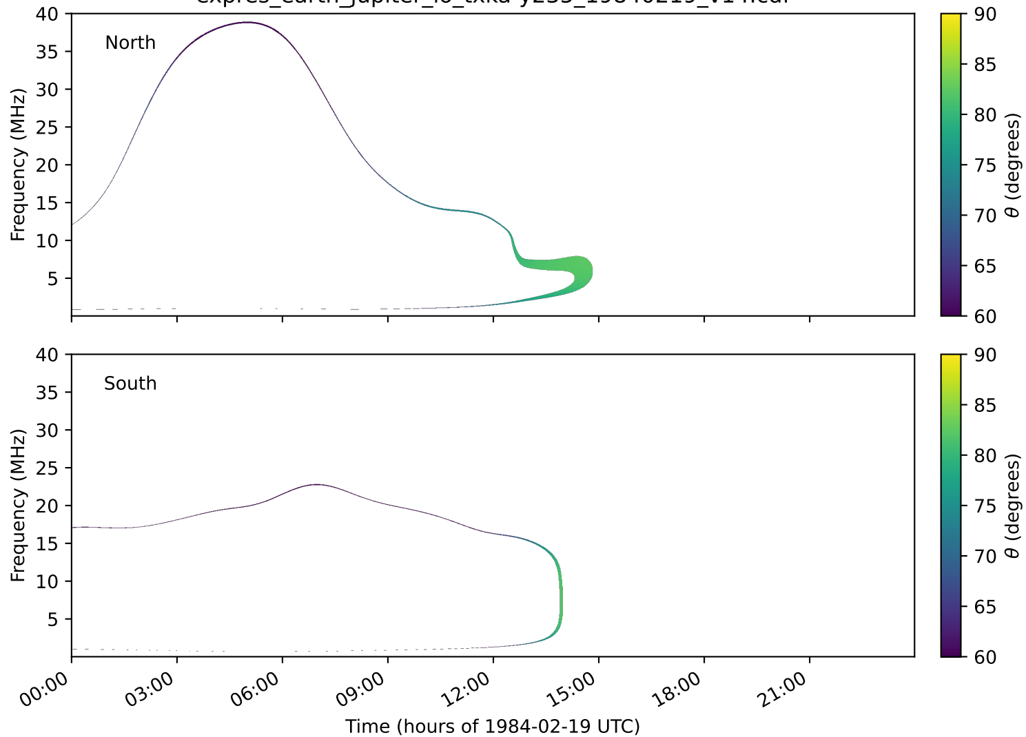
expres_earth_jupiter_io_txka-y235_19840219_v14.cdf
