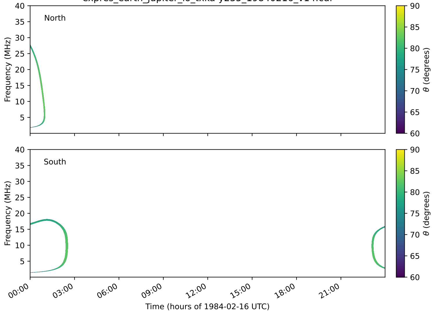
expres_earth_jupiter_io_txka-y235_19840216_v14.cdf
