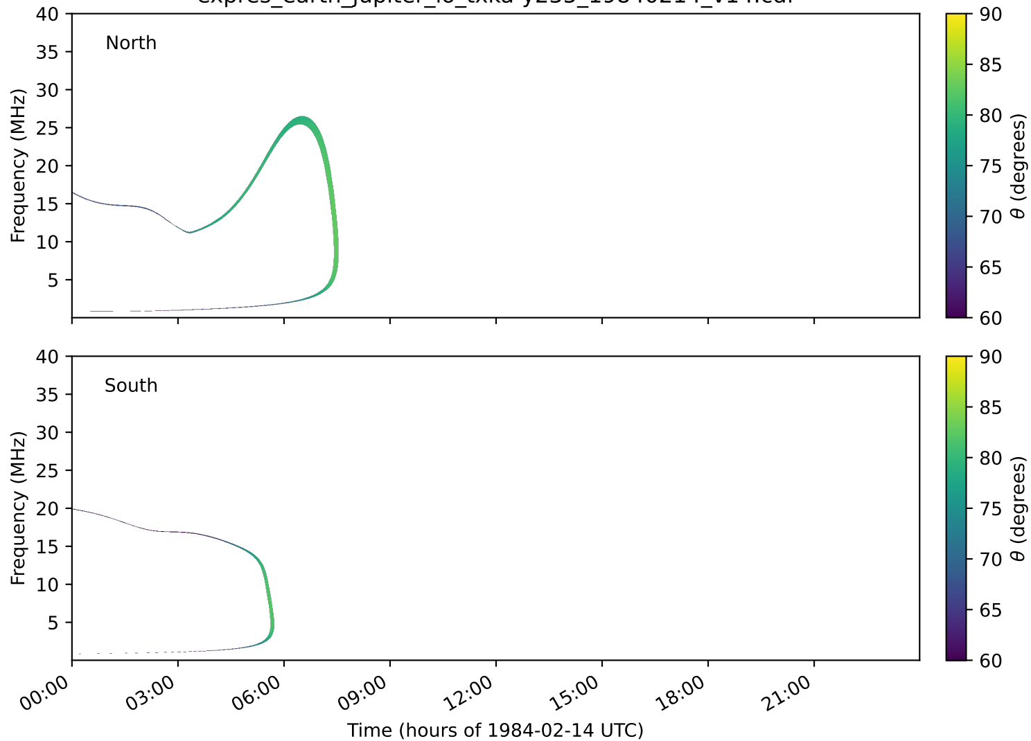
expres_earth_jupiter_io_txka-y235_19840214_v14.cdf
