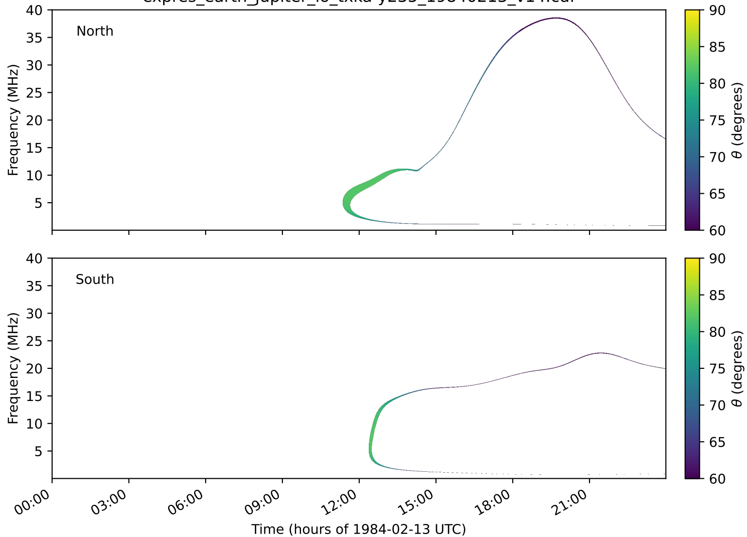
expres_earth_jupiter_io_txka-y235_19840213_v14.cdf
