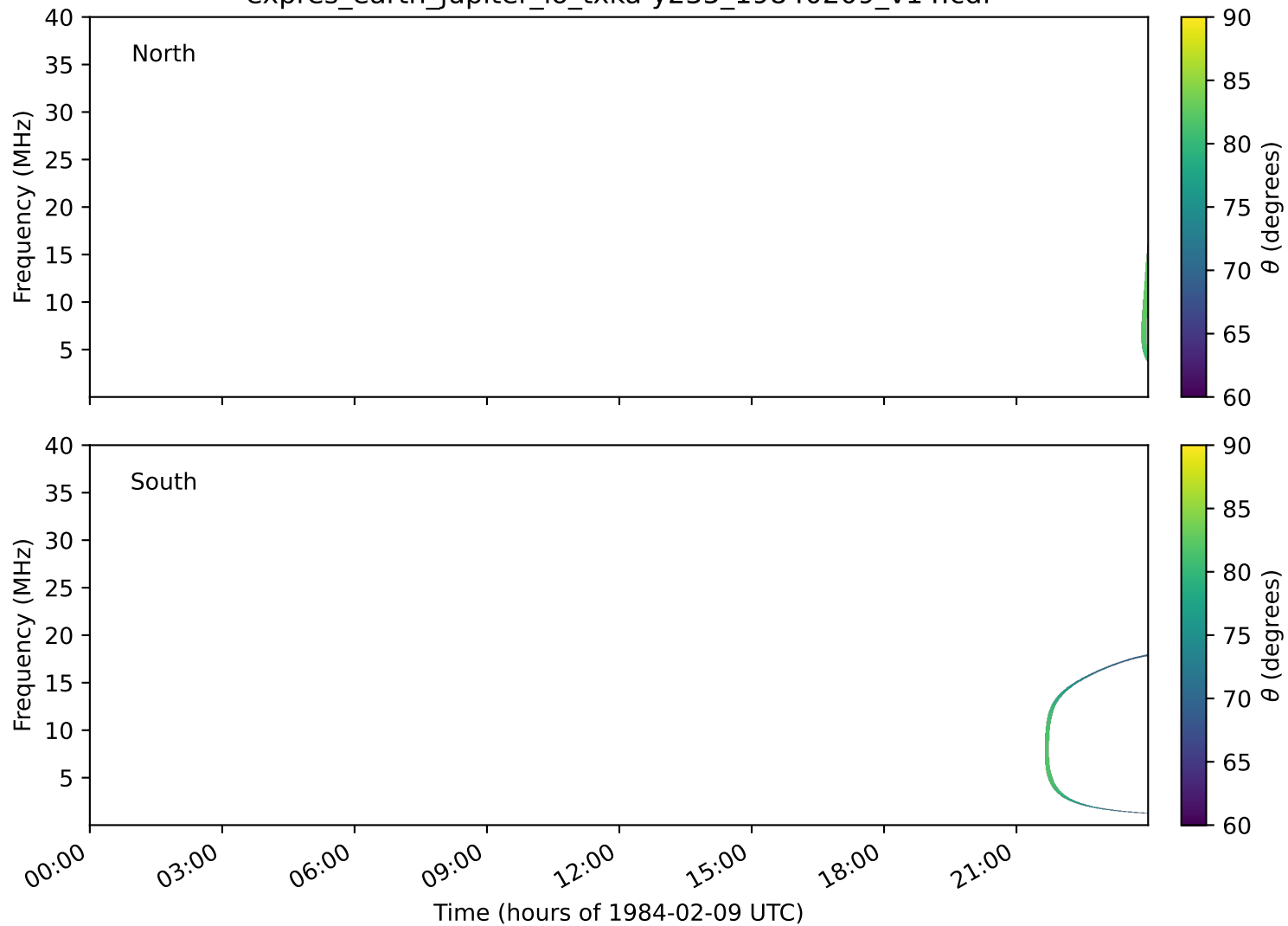
expres_earth_jupiter_io_txka-y235_19840209_v14.cdf
