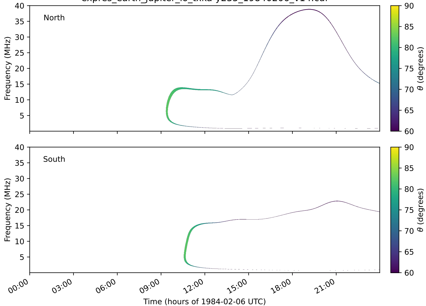
expres_earth_jupiter_io_txka-y235_19840206_v14.cdf
