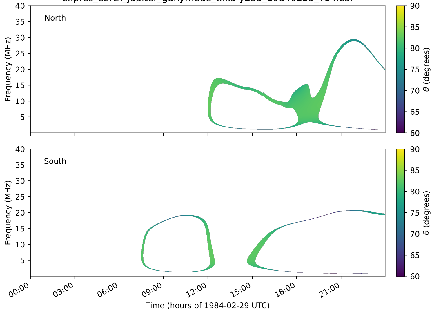
expres_earth_jupiter_ganymede_txka-y235_19840229_v14.cdf
