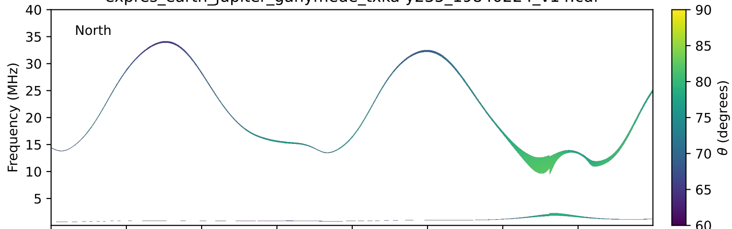
expres_earth_jupiter_ganymede_txka-y235_19840224_v14.cdf
