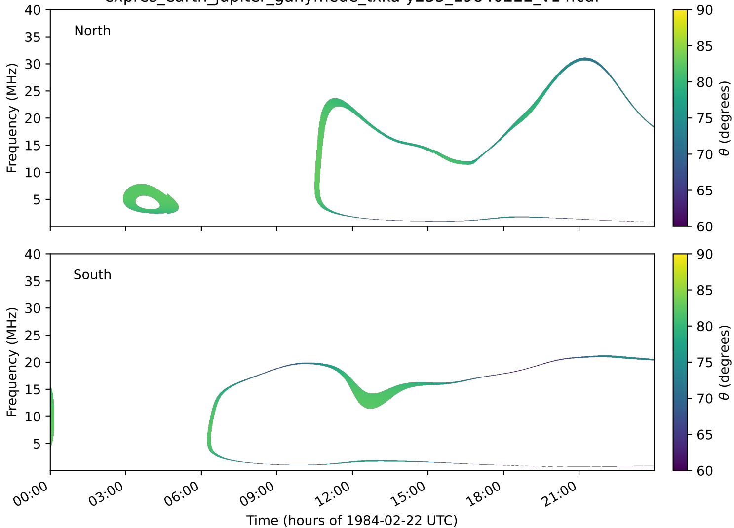
expres_earth_jupiter_ganymede_txka-y235_19840222_v14.cdf
