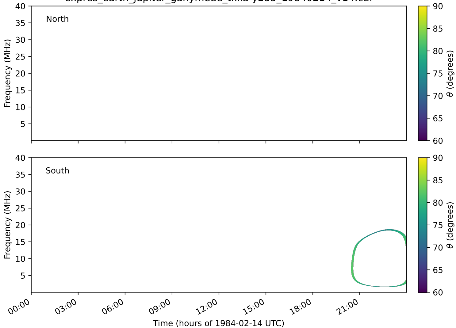
expres_earth_jupiter_ganymede_txka-y235_19840214_v14.cdf
