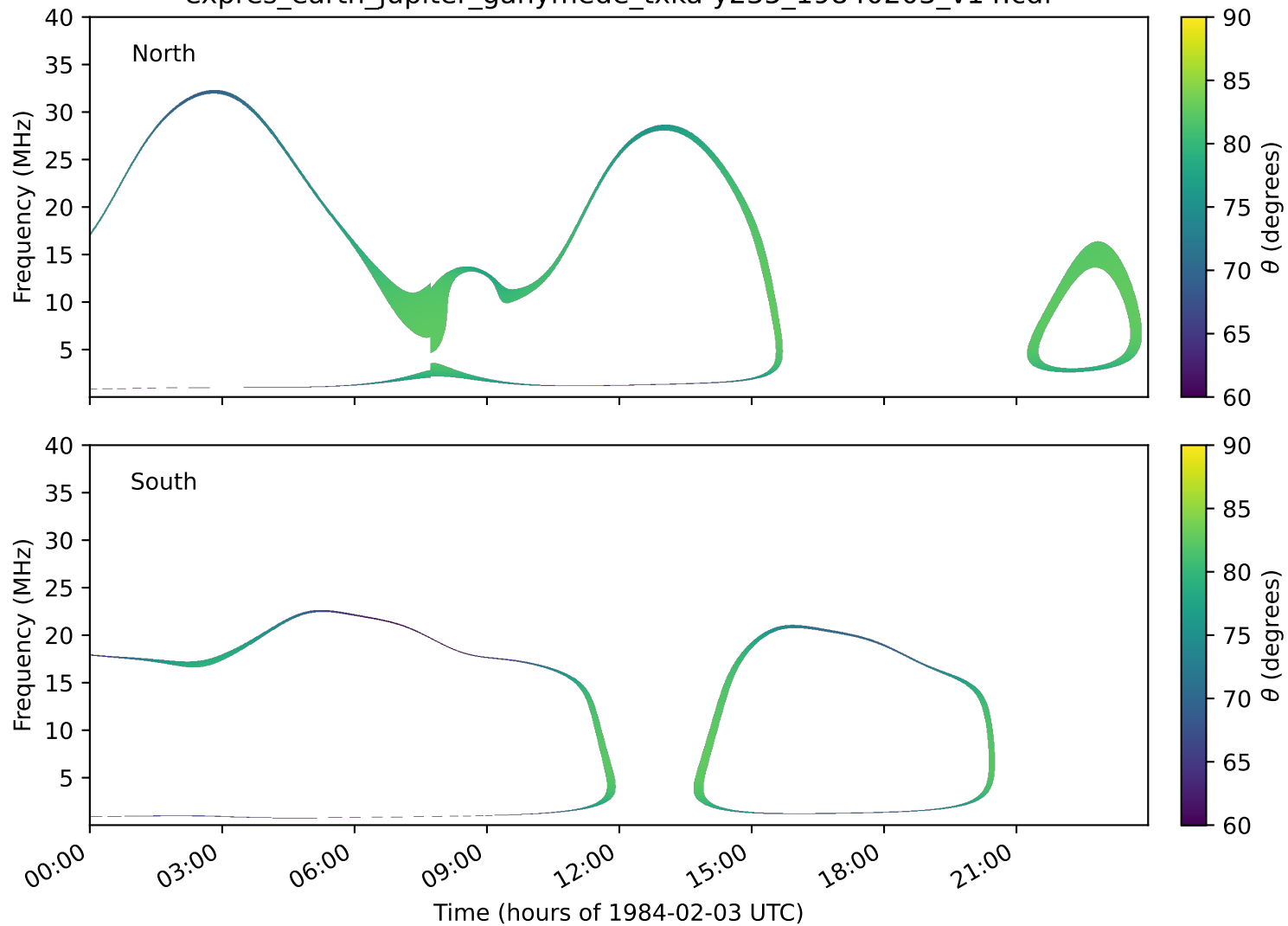
expres_earth_jupiter_ganymede_txka-y235_19840203_v14.cdf
