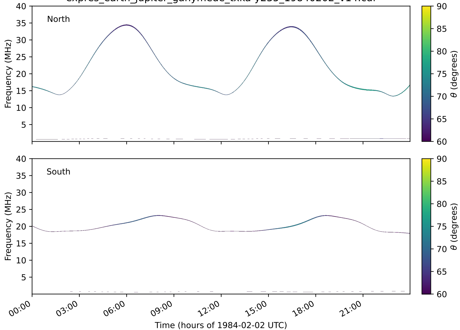
expres_earth_jupiter_ganymede_txka-y235_19840202_v14.cdf
