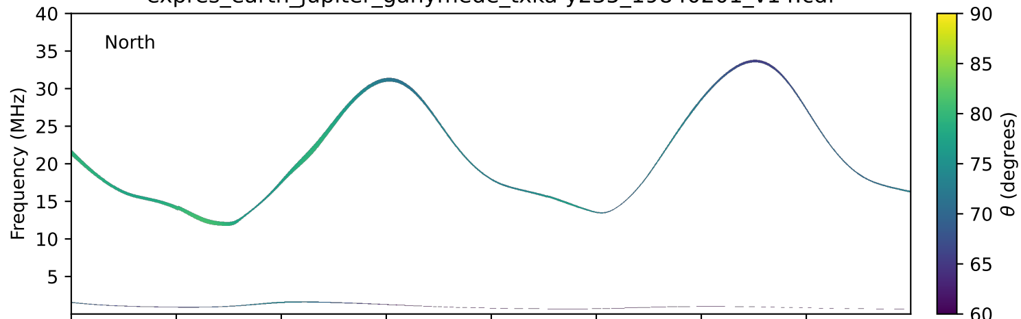
expres_earth_jupiter_ganymede_txka-y235_19840201_v14.cdf
