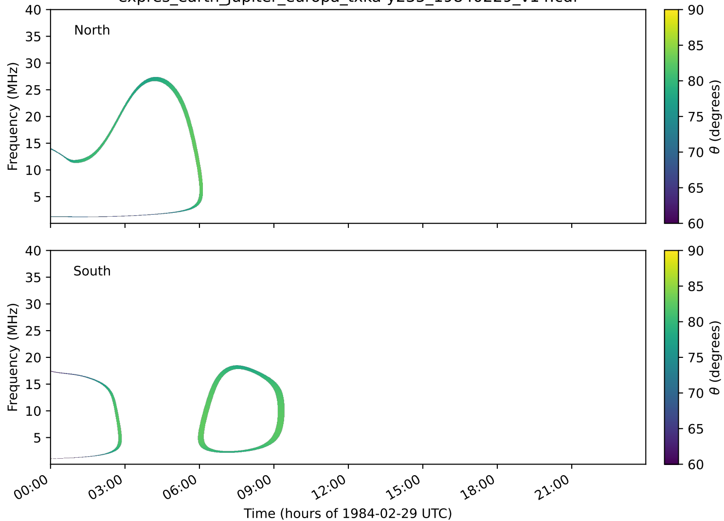
expres_earth_jupiter_europa_txka-y235_19840229_v14.cdf
