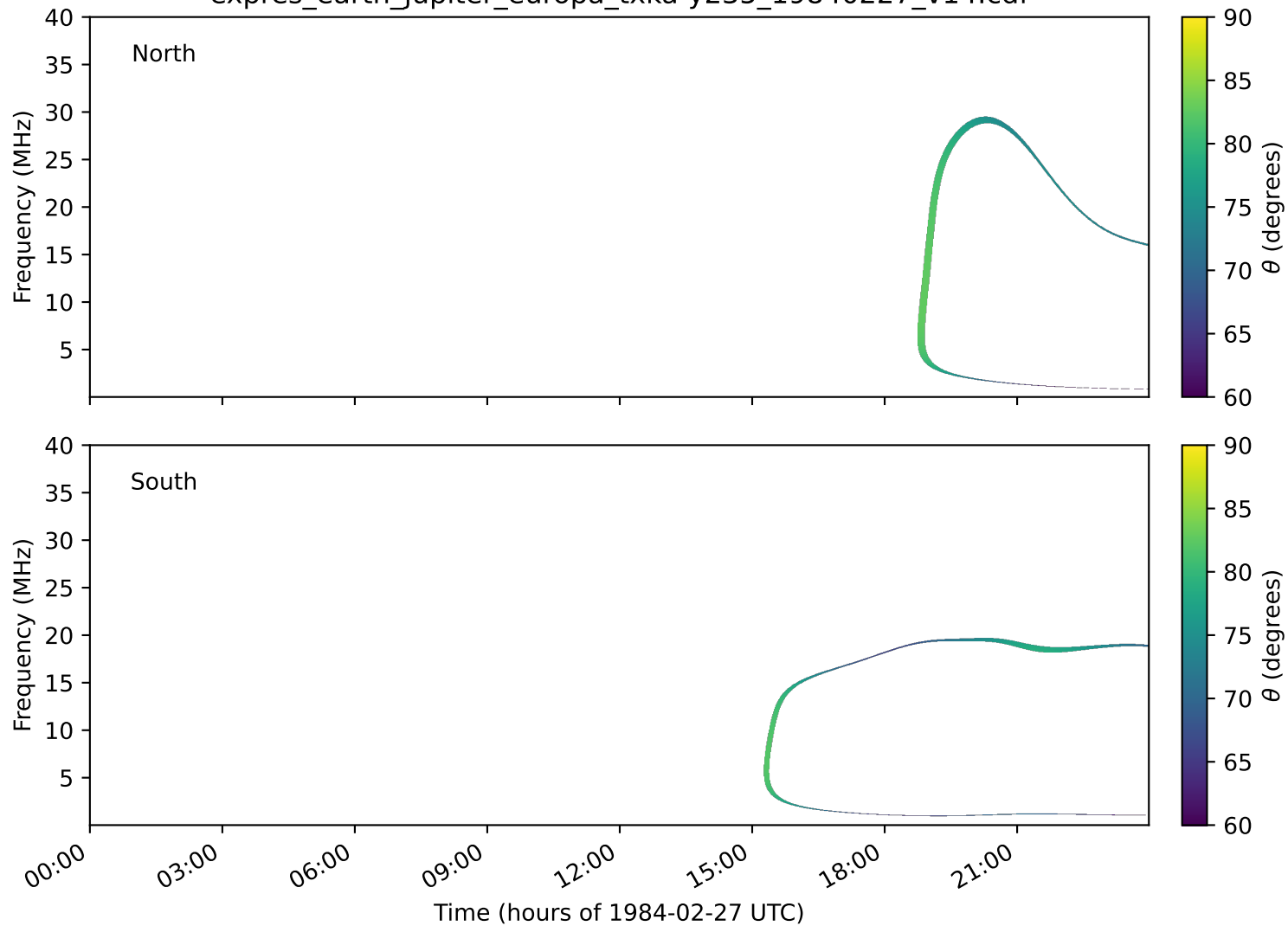
expres_earth_jupiter_europa_txka-y235_19840227_v14.cdf
