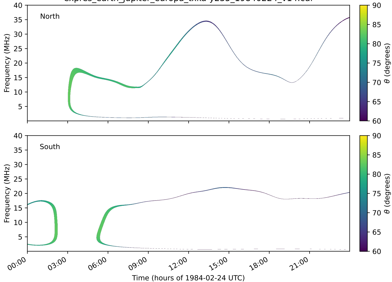
expres_earth_jupiter_europa_txka-y235_19840224_v14.cdf
