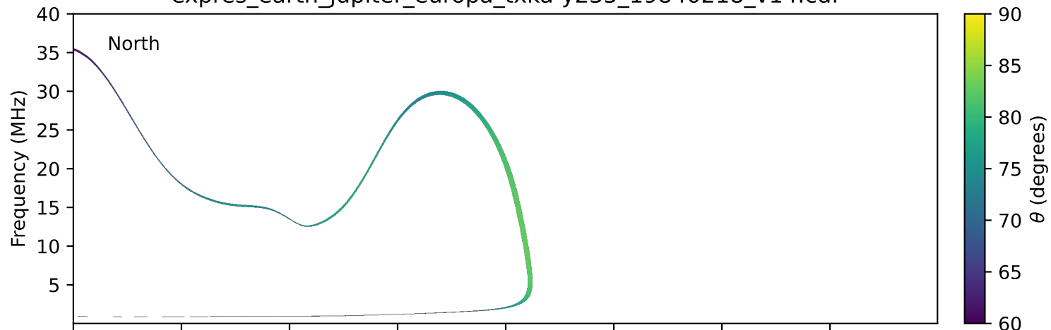
expres_earth_jupiter_europa_txka-y235_19840218_v14.cdf
