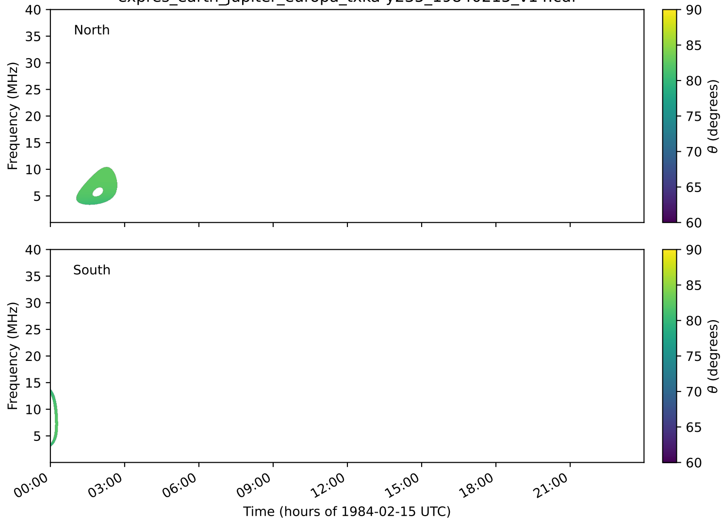
expres_earth_jupiter_europa_txka-y235_19840215_v14.cdf
