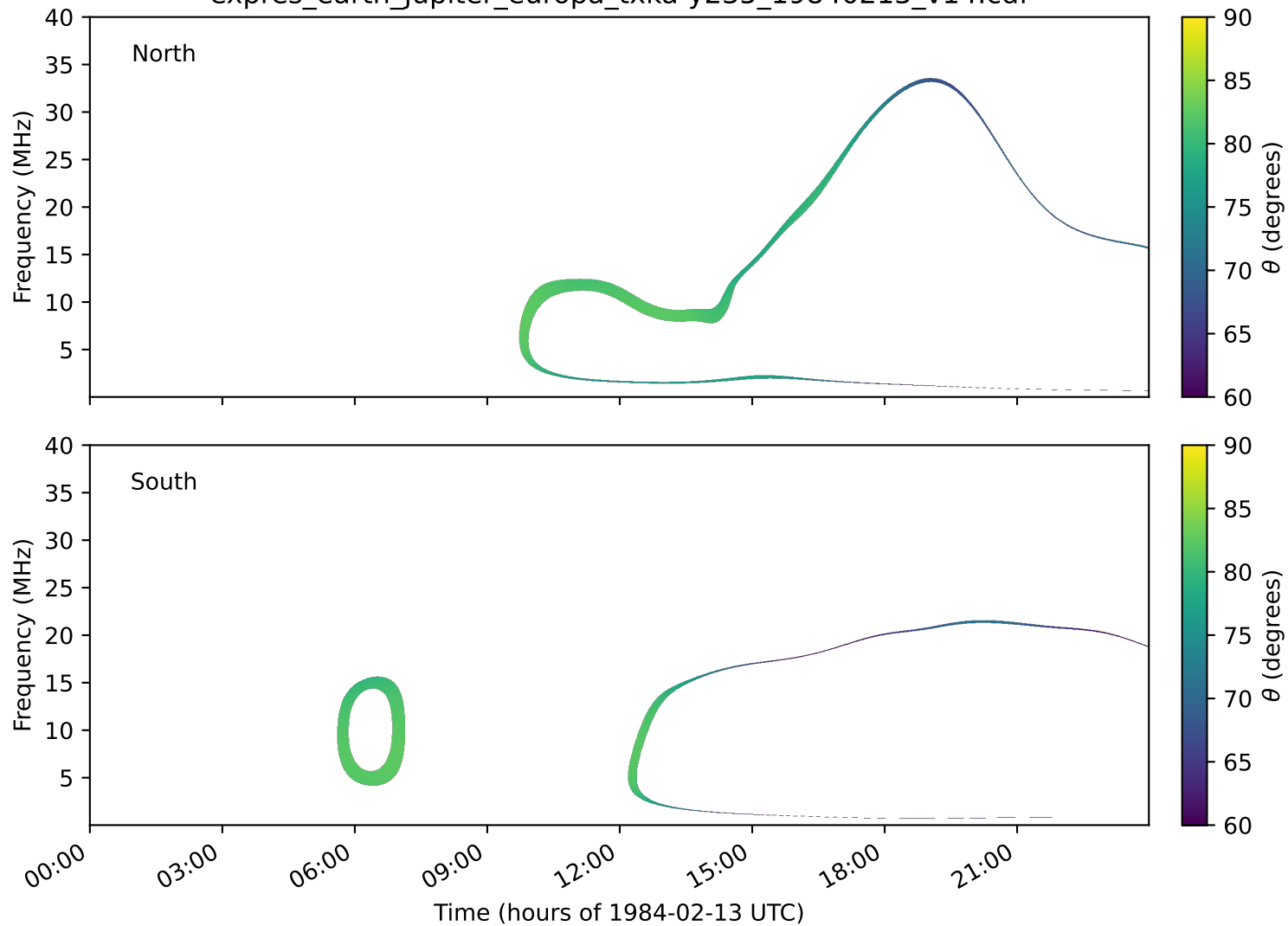
expres_earth_jupiter_europa_txka-y235_19840213_v14.cdf
