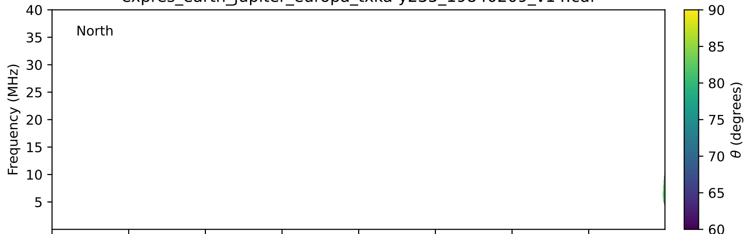
expres_earth_jupiter_europa_txka-y235_19840209_v14.cdf
