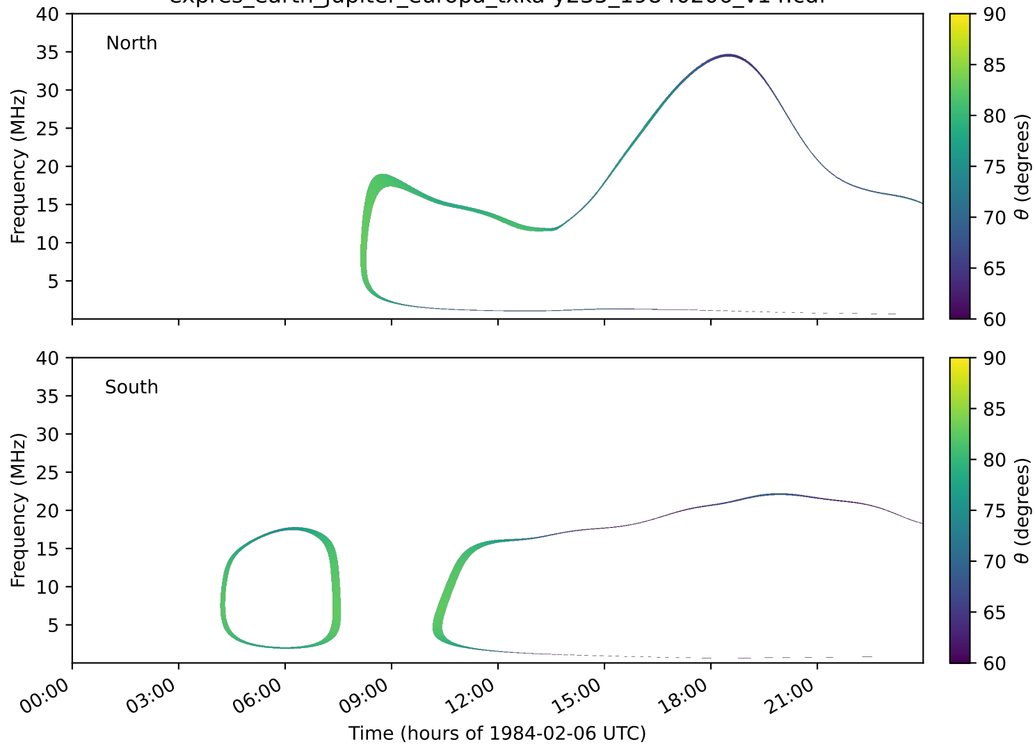
expres_earth_jupiter_europa_txka-y235_19840206_v14.cdf
