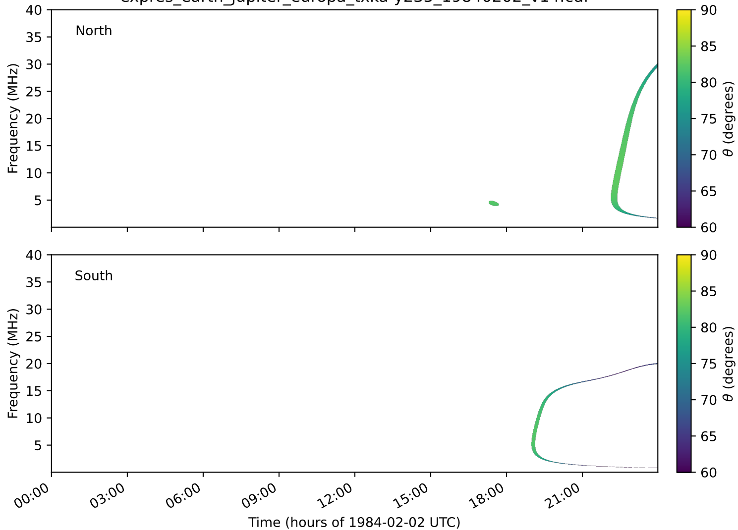
expres_earth_jupiter_europa_txka-y235_19840202_v14.cdf
