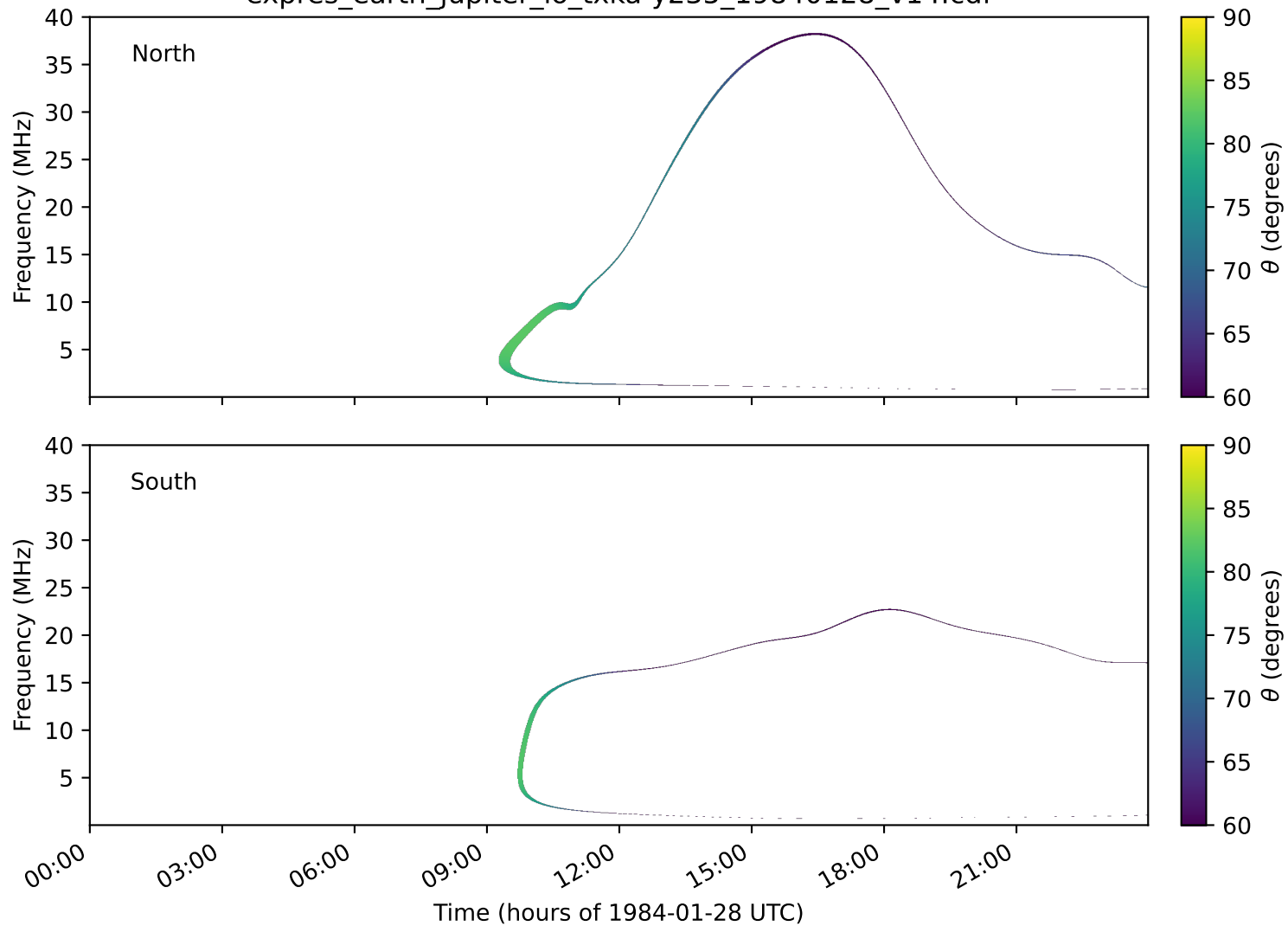
expres_earth_jupiter_io_txka-y235_19840128_v14.cdf
