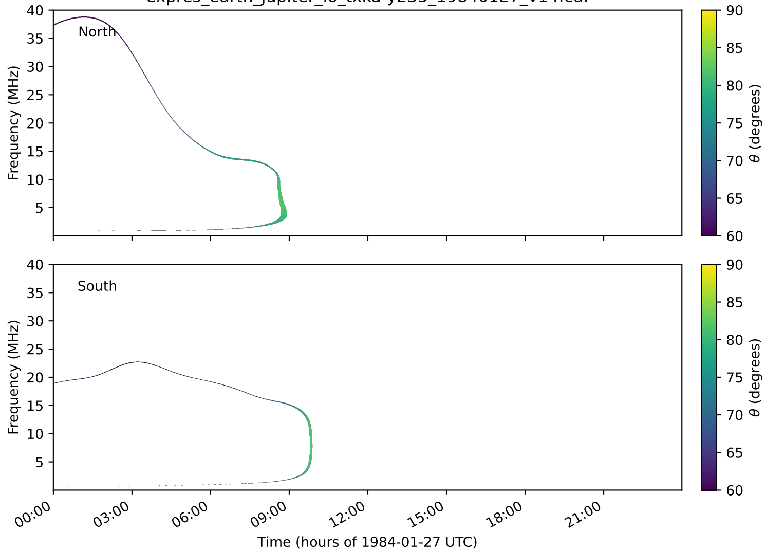
expres_earth_jupiter_io_txka-y235_19840127_v14.cdf
