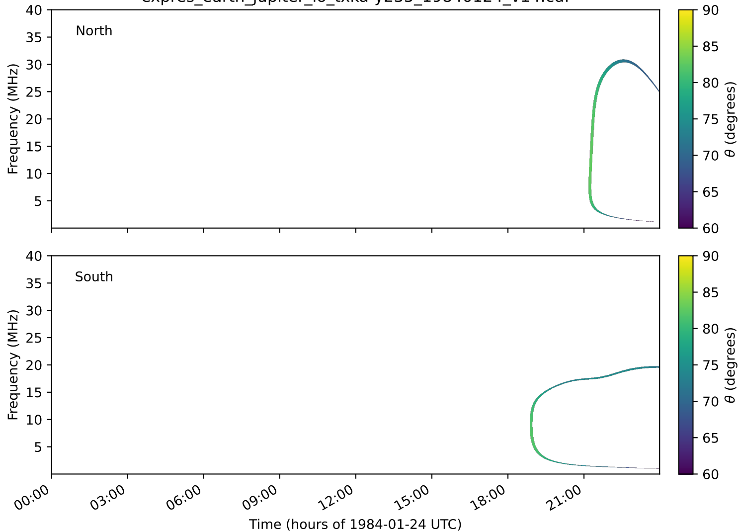
expres_earth_jupiter_io_txka-y235_19840124_v14.cdf
