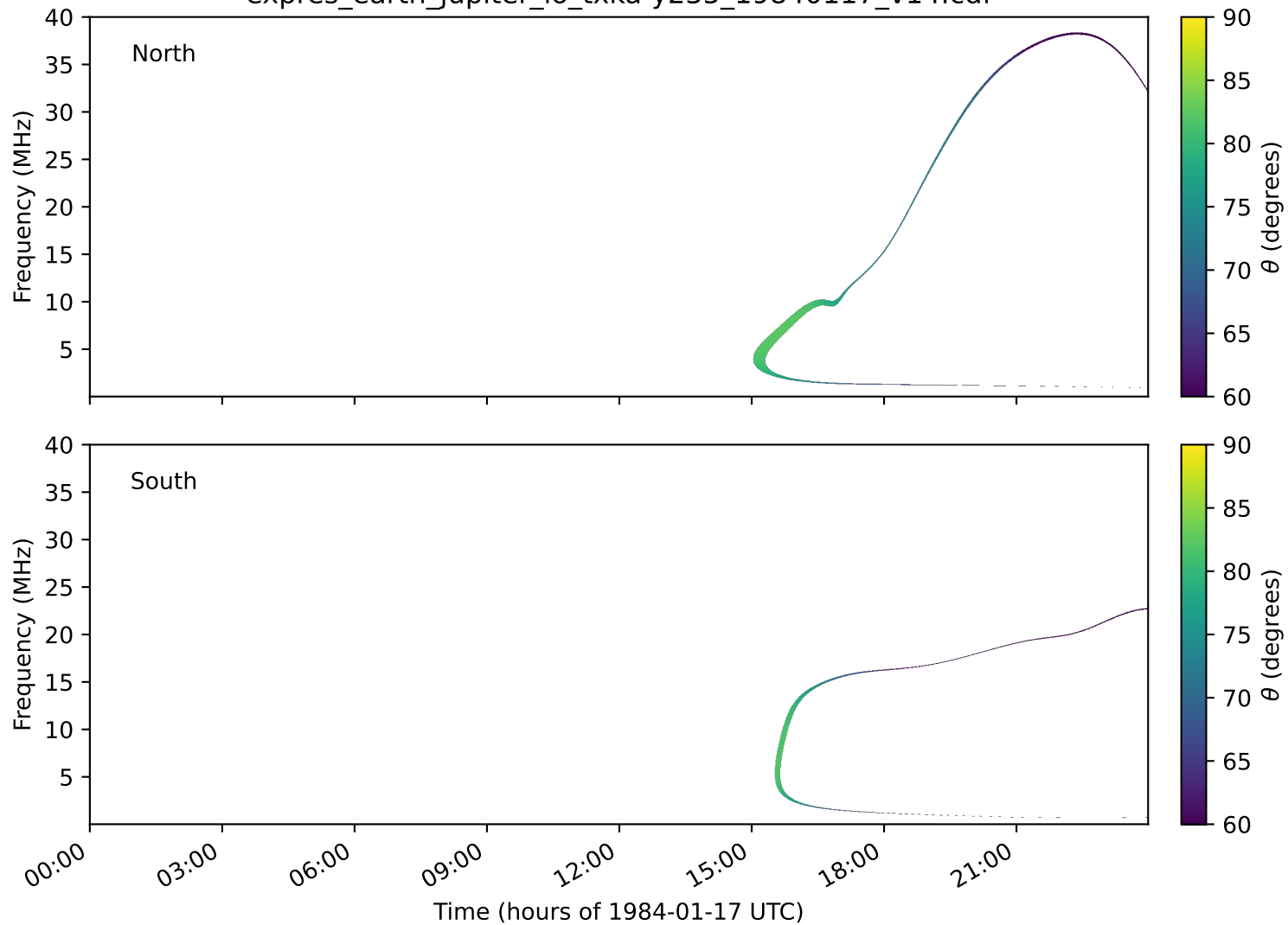
expres_earth_jupiter_io_txka-y235_19840117_v14.cdf
